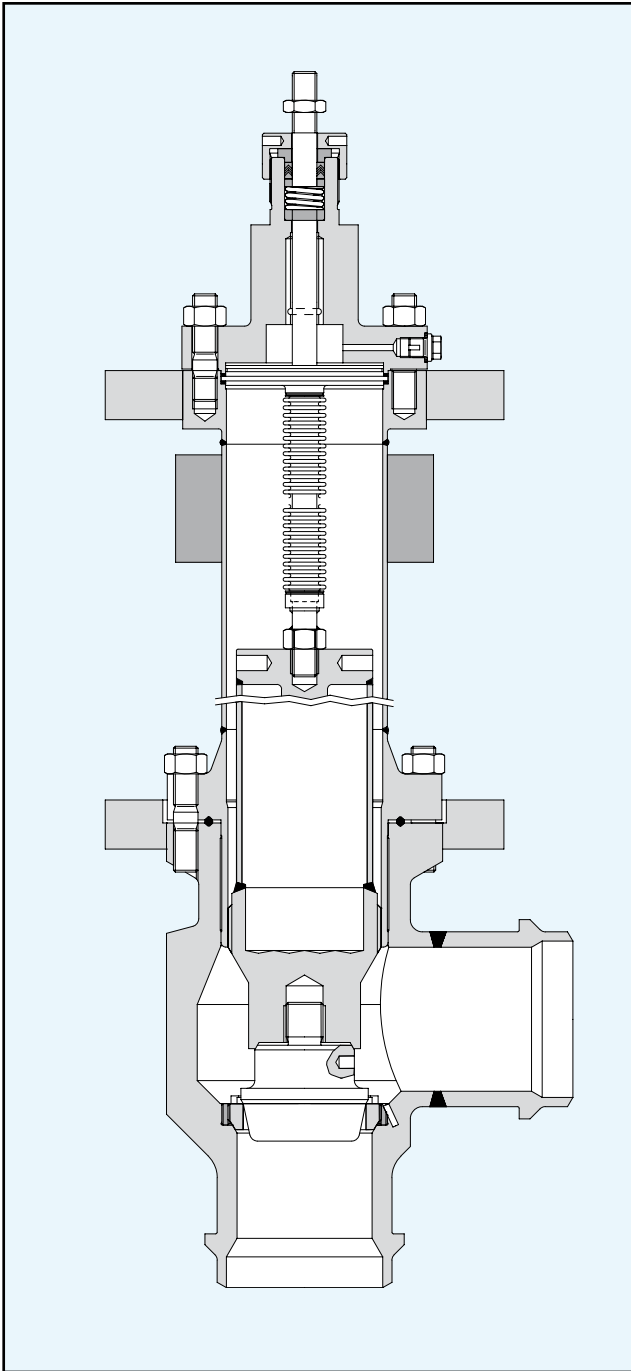
Low temperature valve with bellows seal and test connection
