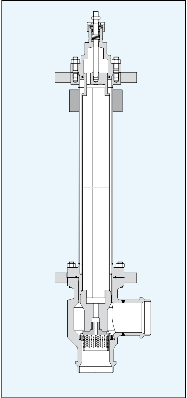
Low temperature valve with pressure balancing and multi-hole cage plug
