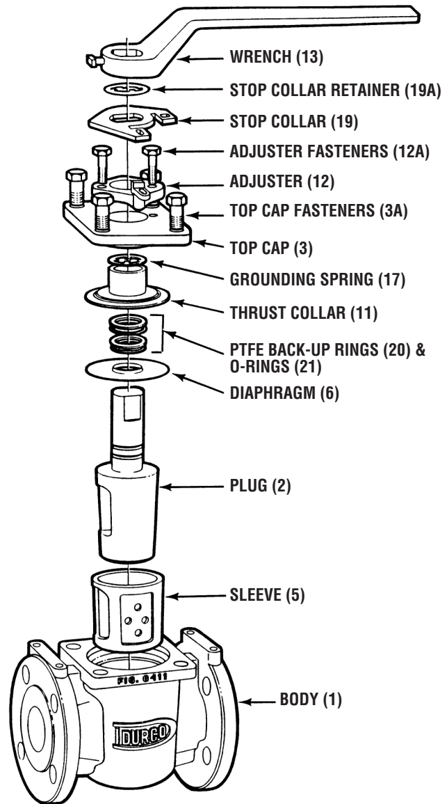
FIGURE II-1 TYPICAL ASSEMBLY OF G4 MARATHON AND G4R MARATHON VALVE
