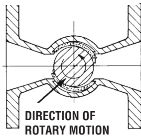
FIGURE V B-2A Optional assembly operation for 1" & 1 1/2" G-4 Valves
