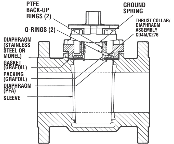
G4Z & G4ZH FIREPROOF VALVE
