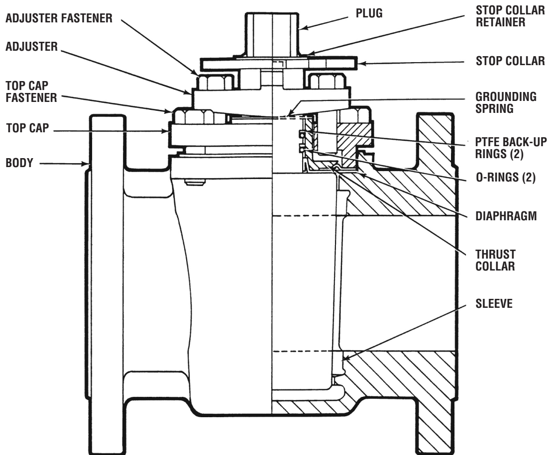
FIGURE V A-10 ASSEMBLED VALVE
