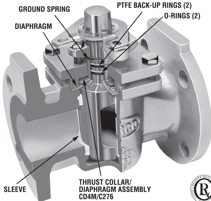
G4 MARATHON VALVE
