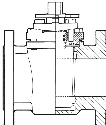
FIGURE VI-9 ASSEMBLED G4Z MARATHON & G4ZHF MARATHON
