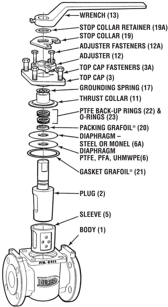
FIGURE VI-1 TYPICAL ASSEMBLY OF G4Z MARATHON AND G4ZHF MARATHON
