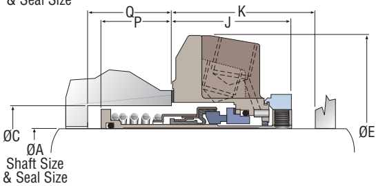
ISC1EX Single Elastomer Bellows*
