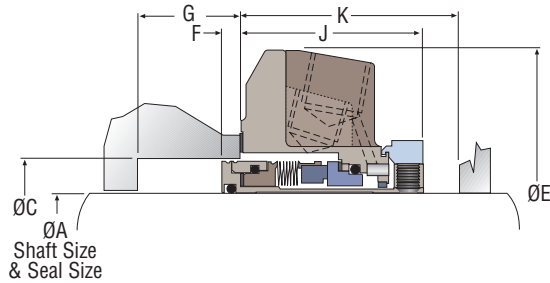
ISC1BX Single Metal Bellows
