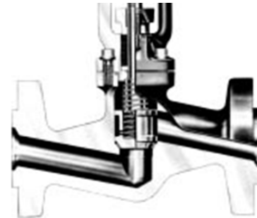
Figure 846: Typical Stop-Check Valve with Body-Guided Disk
