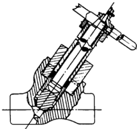
Lapping with Valve Disk Assembly
