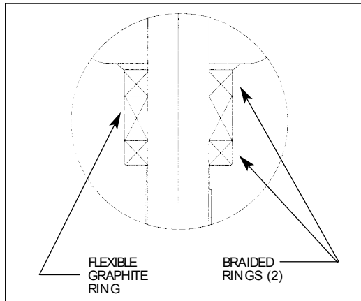
Packing Chamber Schematic
