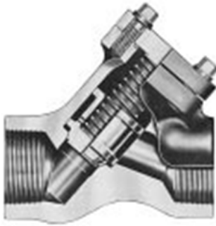
Figure 838: Bolted Cover Piston Check
