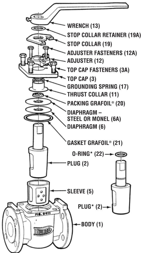
FIGURE VI-1A TYPICAL ASSEMBLY OF G4Z AND G4ZHF
