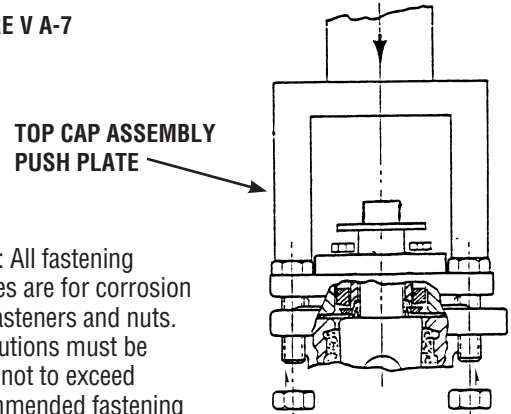
ASSEMBLE TOP CAP ASSEMBLY OVER PLUG AND PUSH INTO BODY
