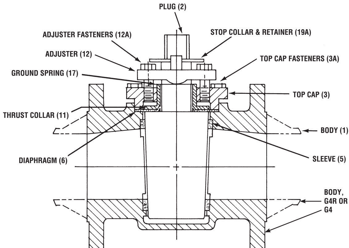
FIGURE V B-7 ASSEMBLED G4 OR G4R VALVE
