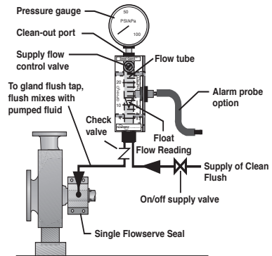
Typical Seal Gard
