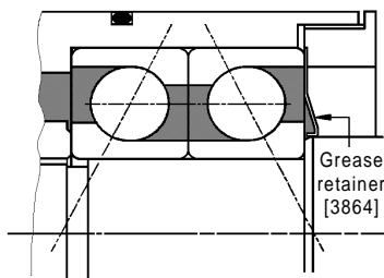
Grease retainer (clearance type) is only fitted on grease lubricated units
