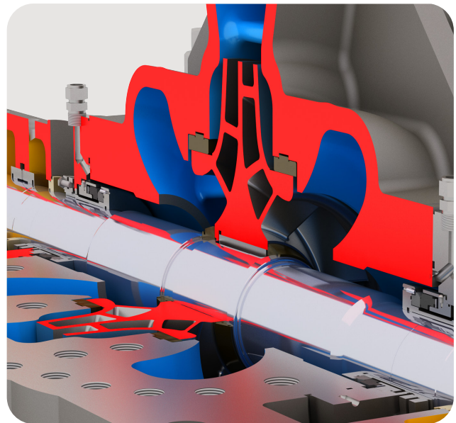
Double volute, axially split casing design minimizes radial hydraulic forces in any condition down to the minimum flow.
