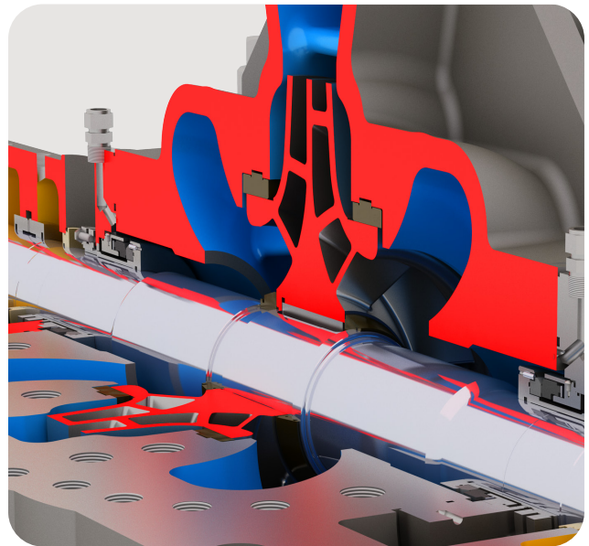
Double volute, axially split casing design minimizes radial hydraulic forces in any condition down to the minimum flow.
